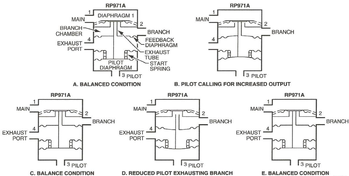
Fig. 4. Typical RP971A Operation.
