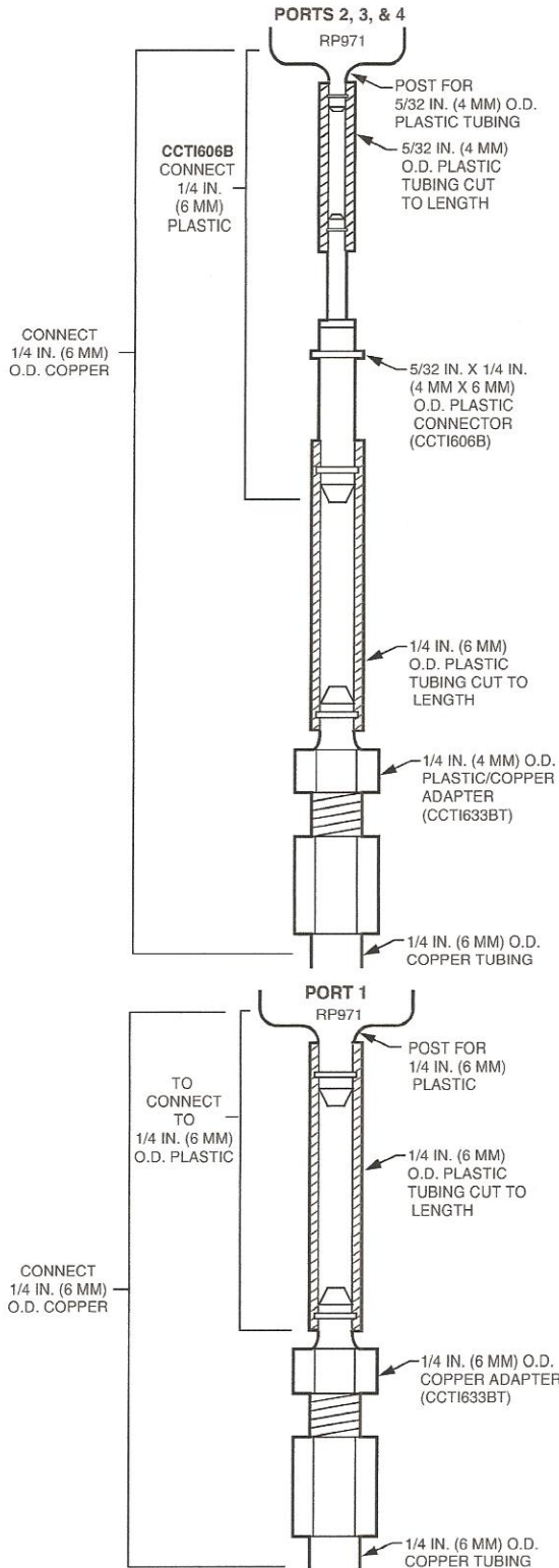
Fig. 3. Adaptation Piping.
