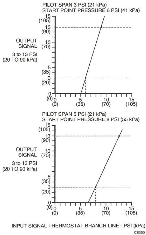
Fig. 5. Graphical Examples of 3 and 5 psi (21 and 34 kPa) models.
