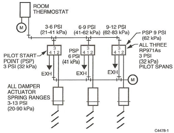
Fig. 6. Typical RP971A Application to Sequence Dampers from a Single Thermostat.
