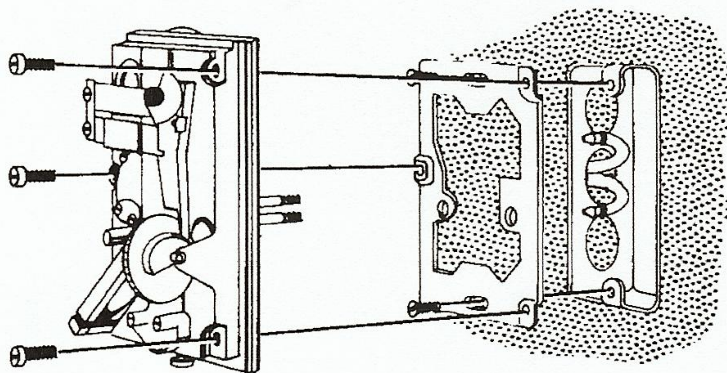
Figure-4 Typical Mounting Thermostat to Electric Box.
