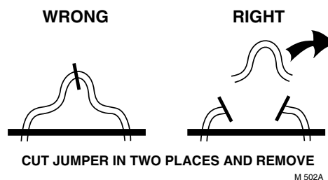
Fig. 13—Proper way to clip out jumper.
