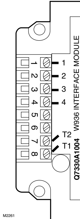
Fig. 9—Q7330A terminals.
