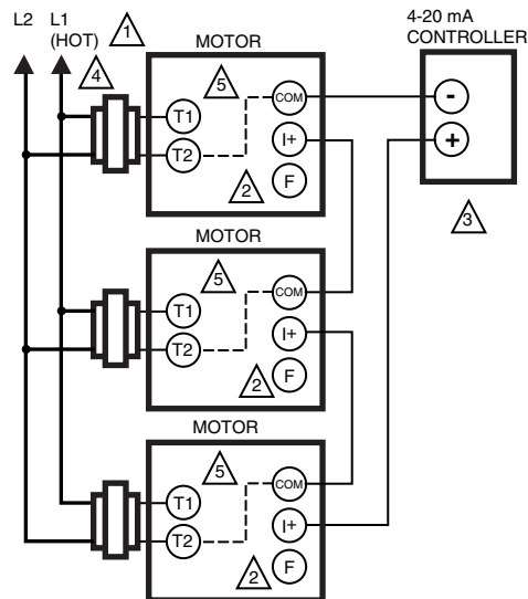
Fig. 7—Typical wiring diagram for Q7230A Interface Module and M91XXX Modutrol IV Motor with 4-20 mA controller.
