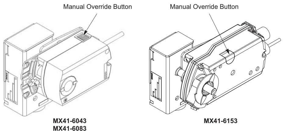
Figure-19 Manual Override Button on MX41-6XX3 Actuators.
