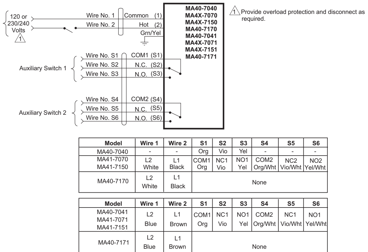
Figure-2 Typical Wiring Diagram for 120 Vac MA4X-7XXX, and 230/240 Vac MA4X-7XXX Two Position Actuators.
