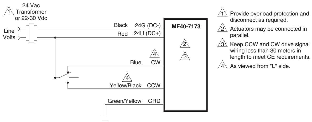
Figure-6 Typical Wiring Diagram for MF40-7173 Floating Actuators.
