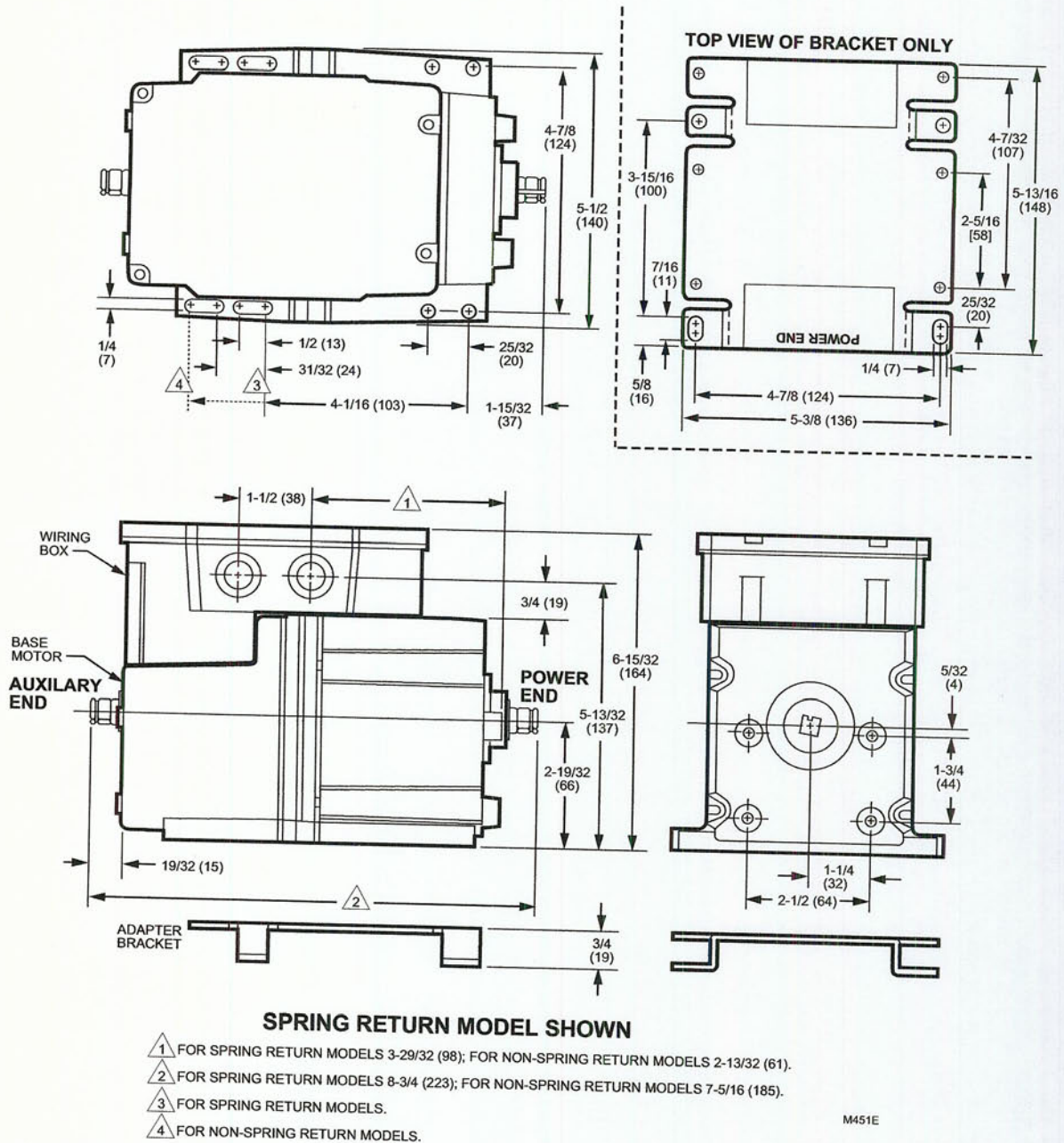
Fig. 1. M7284, M7285, M7294 dimensions in in. (mm). Note: M7281, M7282 models do not have auxiliary shaft. All other dimensions are the same.
