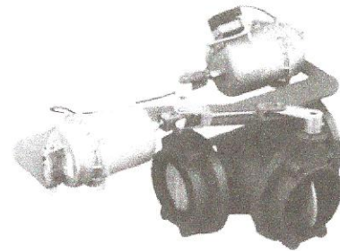
Three-Way VF Butterfly Valve with Tandem D-3246 Actuators
